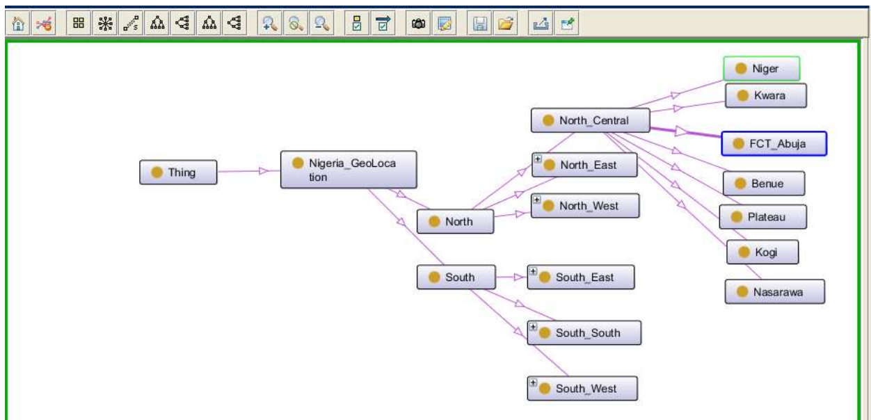
Figure 4.1: Visualization view of the Nigeria Geography Ontology Using OntoGraf
